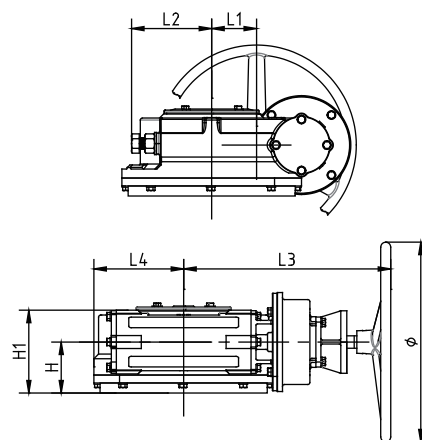
DN550-DN700
