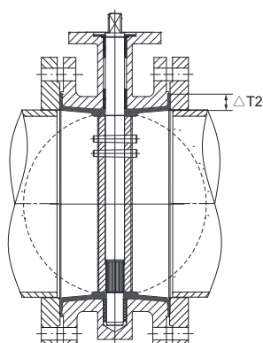
Double-flange type
