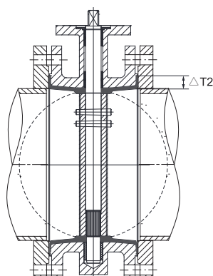
Double-flange type
