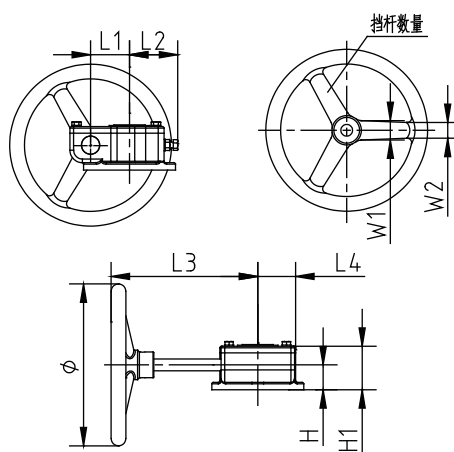
DN50-DN500
