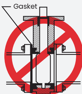
Figure 3 – Initial Centering & Flanging of Valve.
