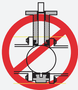
Figure 4 – Final Aligning & Tightening of Flange Bolts
